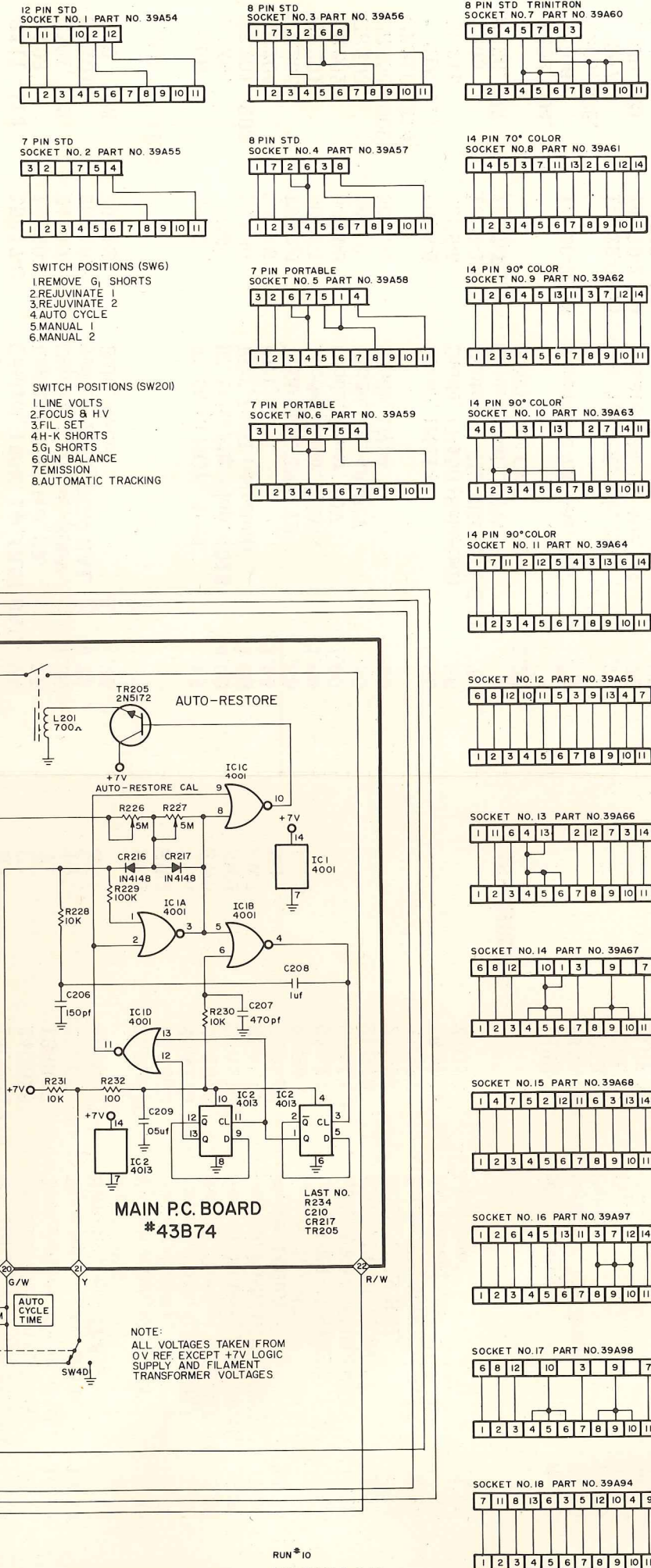
SCHEMATIC DIAGRAM - SUPER MACK CR31A CRT TESTER & BEAM BUILDER
