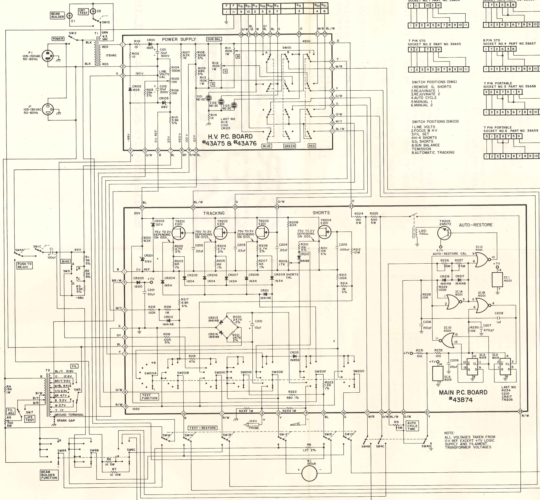
SCHEMATIC DIAGRAM - SUPER MACK CR31A CRT TESTER & BEAM BUILDER
